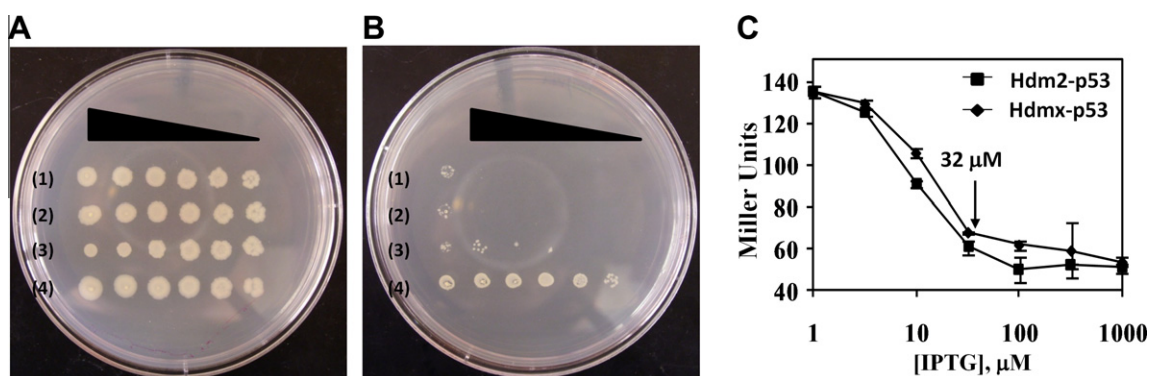
Figure 2. Intracellular analysis of repressor pairs simulating Hdm2-p53 and Hdmx-p53 interactions in the E. coli reporter strain. (A and B) Growth analysis through droplet inoculation of serially diluted strains ( 10^{-10} colony forming units (cfu)) expressing the Hdmx-p53 pair of DBD fusions (row 1), the Hdm2-p53 pair of DBD fusions (row 2), a constitutively active repressor control (row 3) (Ref. 22) and an unrepressed (DBDs only) control (row 4) on a (A) non-selective inducing medium (LB with 100 \mu M IPTG) and (B) selective inducing medium (LB with 100 \mu M IPTG and 25 \mu g/mL kanamycin). (C) Reporter-gene ( \beta -galactosidase) activity analysis of Hdm2-p53 and Hdmx-p53 strains. The arrow indicates the expression level (32 \mu M) for achieving approximately 90% reduction in the reporter expression to be used in the selection procedure.
