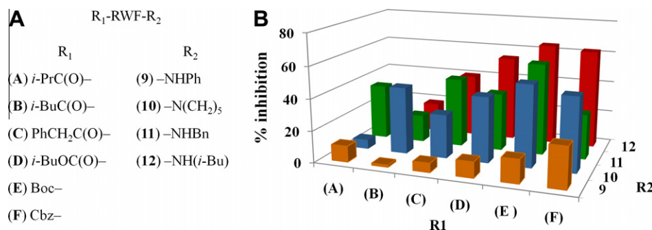
Figure 6. Optimization of the anti-Hdmx inhibitor using a focused library approach. (A) Chemical structures of RWF tripeptide variants with modified termini. (B) Accumulated inhibition profile of the library members at 320 μM (see Table S3 for % inhibition ± SD values). Abbreviations used: i -Pr, isopropyl; i -Bu, isobutyl; Ph, phenyl; Cbz, carbobenzyloxy; Bn, benzyl.
