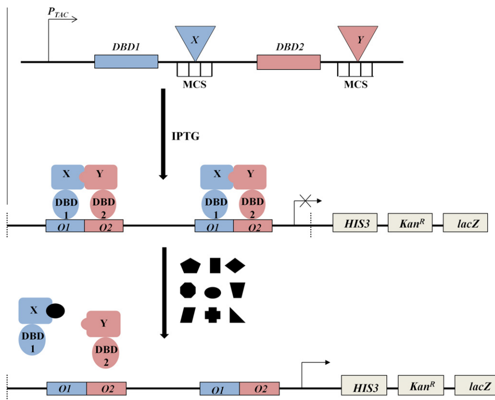
Figure 1. Schematic representation of the genetic system for selection of agents targeting protein–protein interactions. A pair of interacting proteins, designated as X and Y, are inserted downstream of genes coding for DNA-binding domains (DBD1 and DBD2) possessing orthogonal operator affinities (top). Upon induction of P_{TAC} promoter with IPTG, the expressed fusions form a functional heterodimeric repressor that recognizes the corresponding chimeric O1–O2 operator embedded within the promoter region of the tricistronic HIS3 – Kan R – lacZ reporter operon (middle). Perturbation of the repressor complex with an agent selected from a library results in a relief of the promoter blockade and expression of the reporter genes (bottom).
