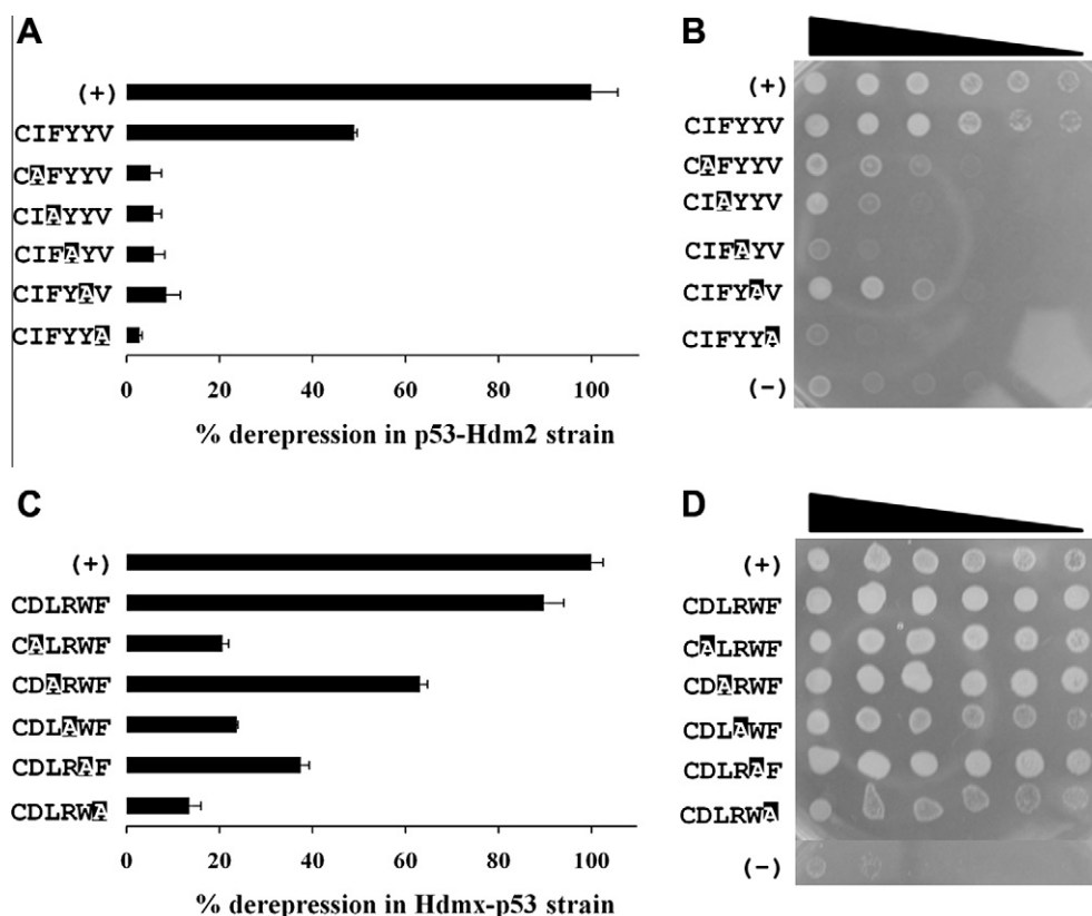
Figure 4. Performance of the selected SICLOPPS constructs and the corresponding single-alanine mutants in the reporter-gene and growth rate assays. (A and B) ONPG assay data and droplet inoculation analysis, respectively, of the anti-Hdm2 CIFYYV construct and its mutants in the Hdm2-p53 strain. (C and D) ONPG assay data and droplet inoculation analysis, respectively, of CDLRWF and its mutants in the Hdmx-p53 strain.
