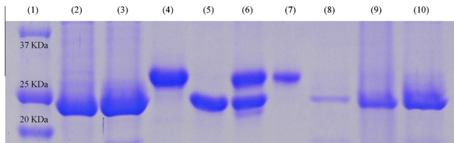
Figure 3. SDS–PAGE analysis of the affinity capture–elution assay performed with the selected SICLOPPS hits. The unspliced constructs containing sequences CIFYYV and CDLRWF were immobilized via chitin-binding domain (CBD) fusion fragments on chitin beads and incubated with an equimolar mixture of Hdm2 or Hdmx (1 mM). Retained materials were subsequently treated with a solution (1 mM) of a p53-derived peptide (ETFSDLWKLL), and the eluate as well as other components of the assay were analyzed by SDS–PAGE. The lane assignments are as follows: lane 1 is a protein ladder; lanes 2 and 3 correspond to the CIFYYV and CDLRWF SICLOPPS constructs, respectively, isolated by chitin beads from crude overexpression lysates; lanes 4 and 5 contain purified Hdm2 and Hdmx, respectively; lane 6 corresponds to an equimolar mixture of Hdm2 and Hdmx; lanes 7 and 8 contain protein material eluted with the p53-derived peptide from the affinity supports containing CIFYYV and CDLRWF leads, respectively, which were pretreated with the equimolar mixture of Hdm2 and Hdmx; lanes 9 and 10 were loaded with the post-elution material retained by the chitin beads pre-functionalized with the CIFYYV and CDLRWF constructs, respectively.
