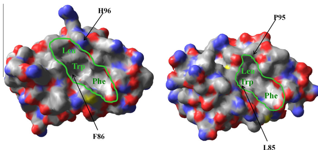
Figure 5. Surface representations of Hdm2 (PDB: 1YCR; left) and Hdmx (PDB: 3DAB; right) in bound states with ligands (p53 residues 15–29) not shown for clarity. The proteins are colored according to the elemental make-up (C, gray; O, red; N, blue; S, yellow). The p53-binding pockets with labeled Leu, Trp and Phe subsites (green) are outlined to highlight the topological differences in the respective binding pockets. The residues proposed to be responsible for differences in ligand recognition patterns (F86 and H96 in Hdm2; L85 and P95 in Hdmx) are indicated by arrows.
